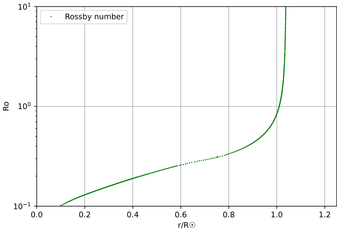
Rossby number, profile 113, age 2.59 \times 10^7
